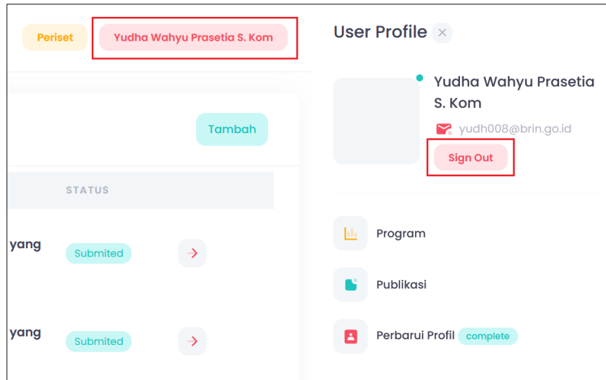
Gambar 17. Halaman Logout
