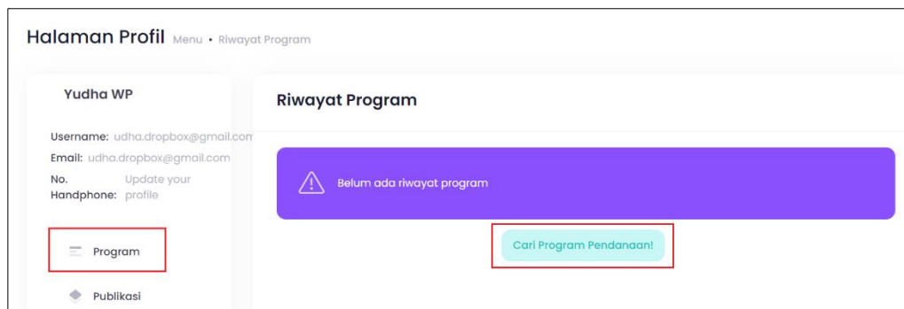
Gambar 9. Halaman Program
